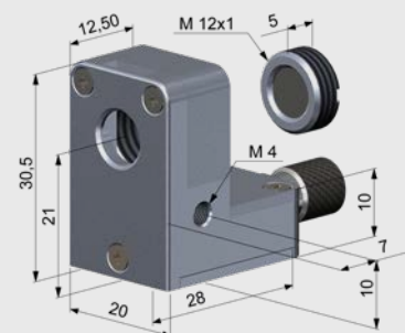
Air purge collar with integrated CF-lens (ACCTAPLCFHT)
