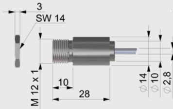
Sensing head
